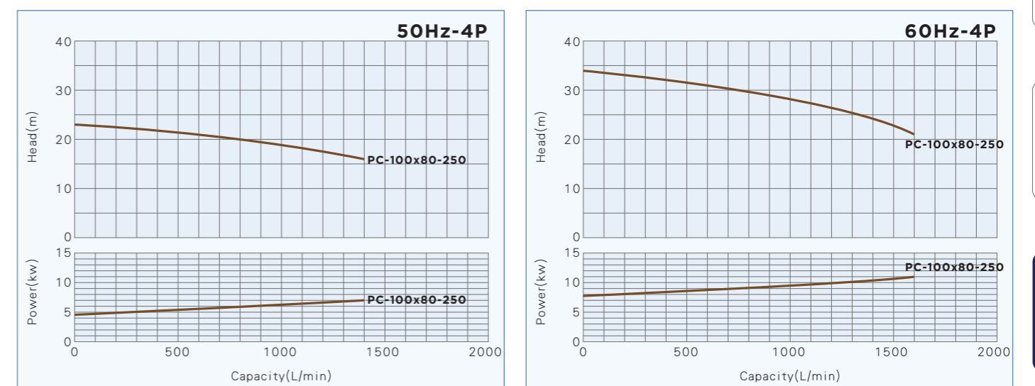
PC-100x80-250
