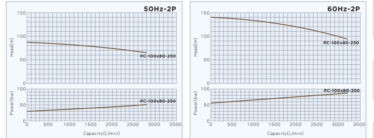
PC-100x80-250
